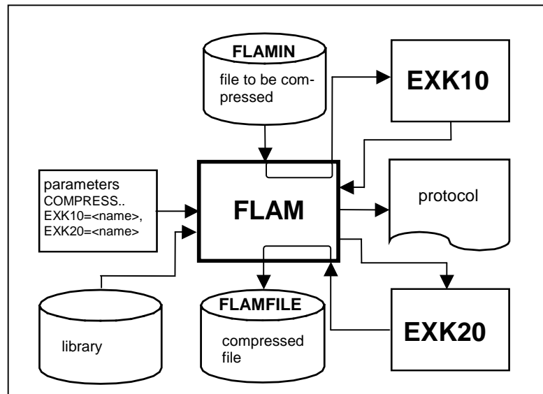
Data flow of compression with user exits
